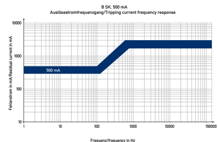
Characteristic B SK 500 mA
