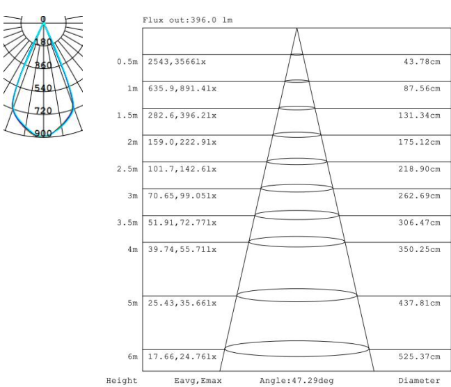
A1055A 12W 4000K Ra97 50D
