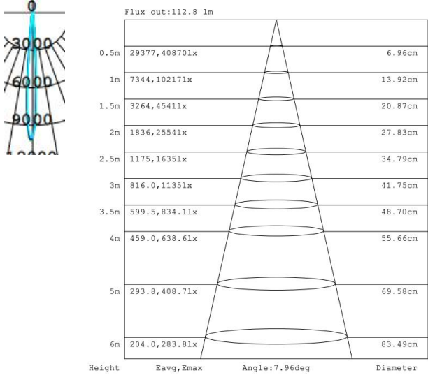
A1055A 12W 4000K Ra97 8D
