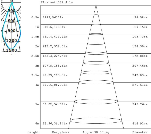
A1055A 12W 4000K Ra97 36D
