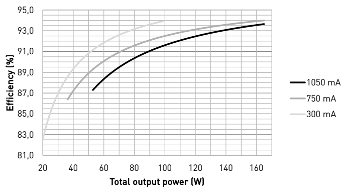
Typical efficiency
