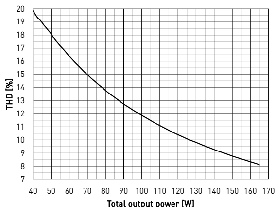
Current THD
