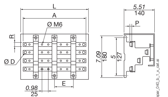
Stair type distribution block, with threaded holes, mounts onto symmetrical DIN rail. Copper bars are factory fitted. Supplied without protection cover.
