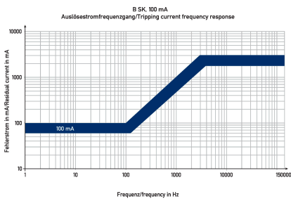
Characteristic B SK 100 mA
