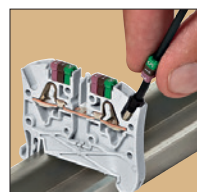
Automatic insertion of flexible wire with ferrule cap or rigid wire up to pitch of 6 mm
