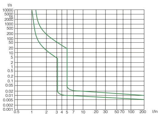
Characteristic B
