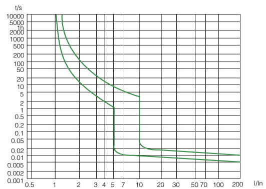
Characteristic C
