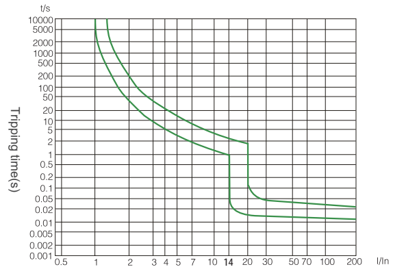
Characteristic K
