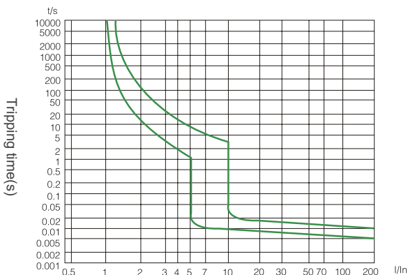
Characteristic C
