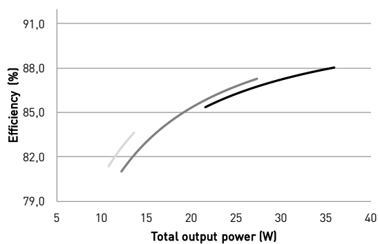
Typical efficiency
